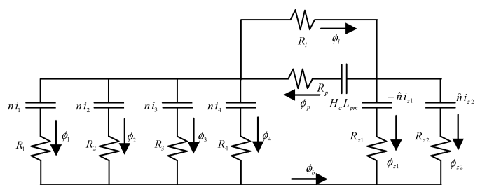
Fig. 2 Equivalent Circuit for a Bidirectional Bearing
