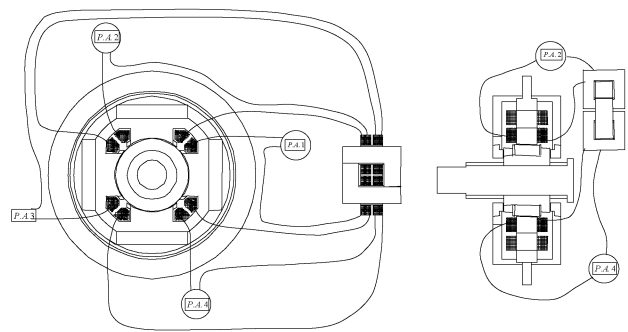
Fig. 1 Schematic of a Bidirectional Magnetic Bearing
